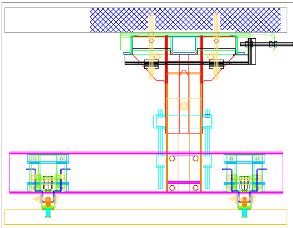
Vertical Anchor System Assembled
